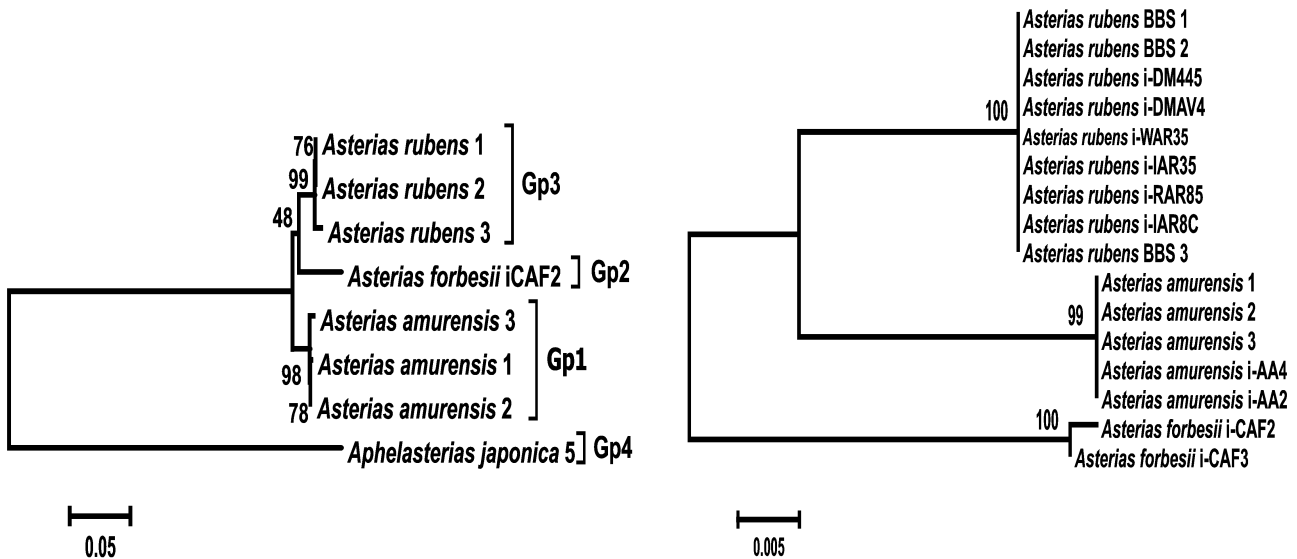
Fig. 4. Phylogenetic tree of the ITS1 , ITS2 , and 5.8S rDNA sequences from starfish of the Asteriidae family. The tree with the maximum logarithm of likelihood ( -4008.5599 ) is shown. The bootstrap values are shown on the branches leading to the corresponding clusters. The lengths of branches are proportional to the number of substitutions. Eight sequences (length, 1600 positions) were analyzed.
