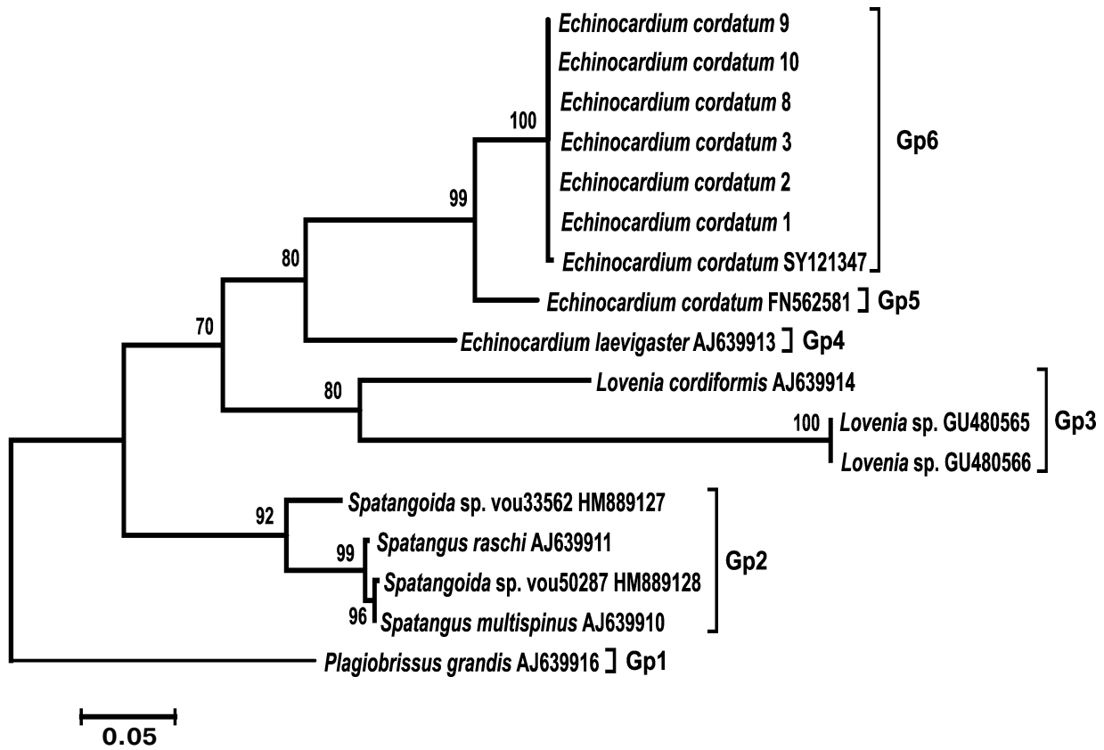
Fig. 3. Phylogenetic tree for the 5'-region of the mitochondrial COI gene from sea urchins of the Loveniidae family. The tree with the maximum logarithm of likelihood ( -2555.0476 ) is shown. The bootstrap values are shown on the branches leading to the corresponding clusters. The lengths of branches are proportional to the number of substitutions. Seventeen sequences (length, 656 positions) were analyzed considering all three codon positions.
