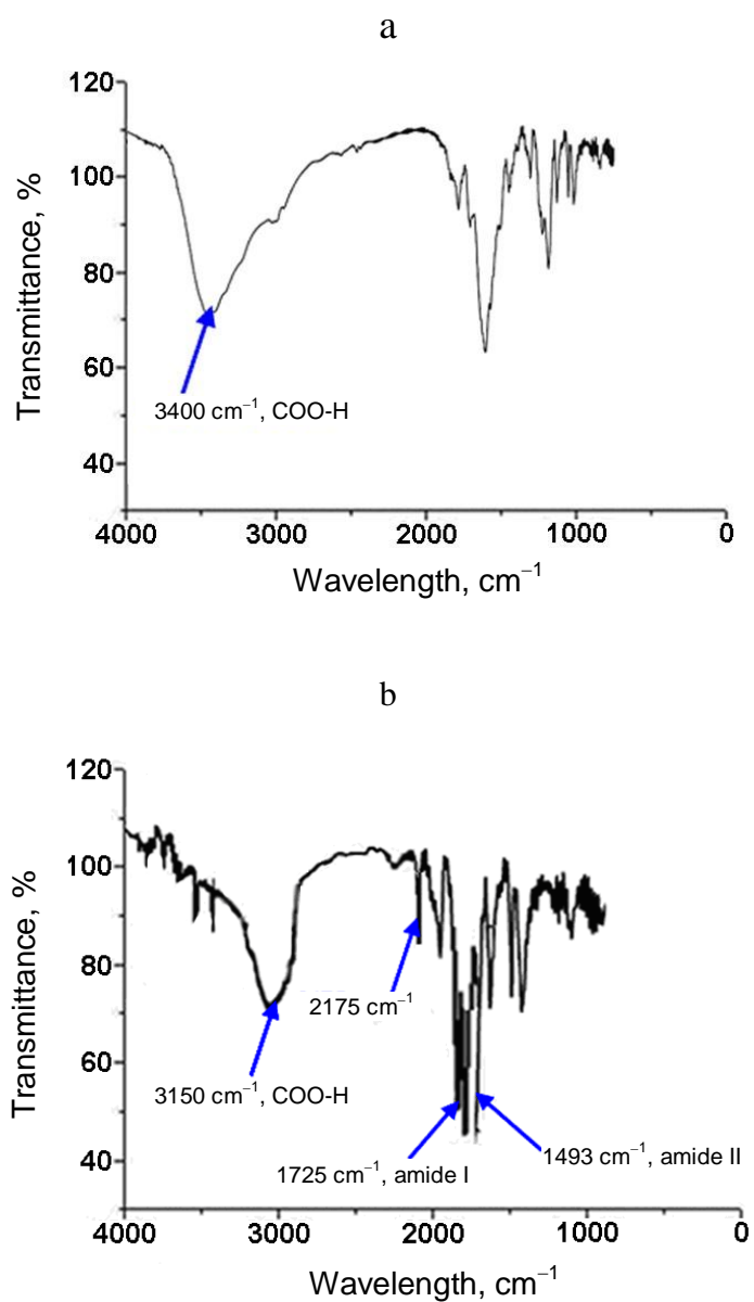
Fig. S1. FT-IR spectra of QD (a) and QD-AL (b).
