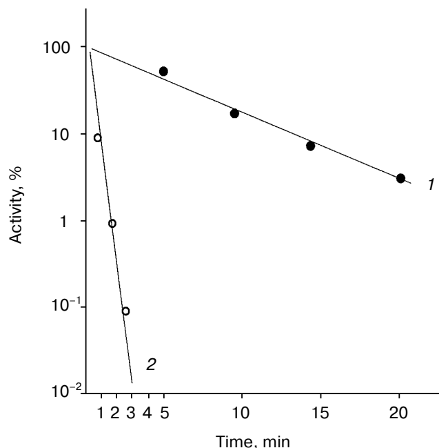
Fig. 1. Kinetics of thermal inactivation of Ph. fischeri and Ph. luminescens luciferases (2 and 1, respectively) in vitro at 43.5°C. The ordinate axis shows the enzymatic activity of luciferase in percent of the initial level. The abscissa axis is the time of thermal inactivation.
